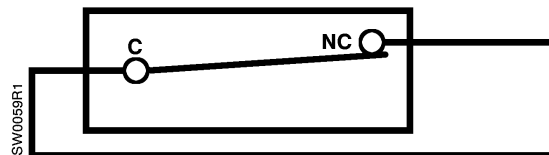
Figure 5. Manual Reset Switch 141-0575.
